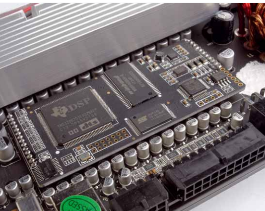
The DSP board contains the large TI DSP, the controller and two memory chips
